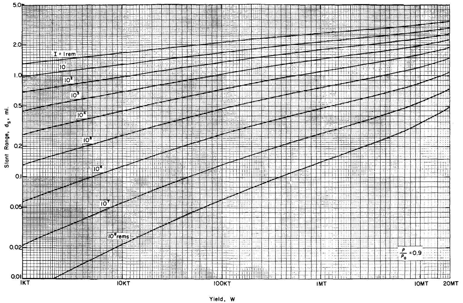
Fig. 2.16—Initial nuclear radiation as a function of slant range and yield for air bursts (see Eq. 2.116).
